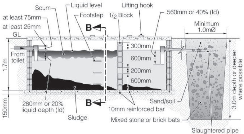
Section on A-A reinforced in unstable soil
