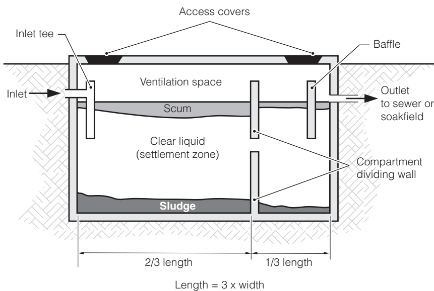
Figure 5.6. Septic-tank
