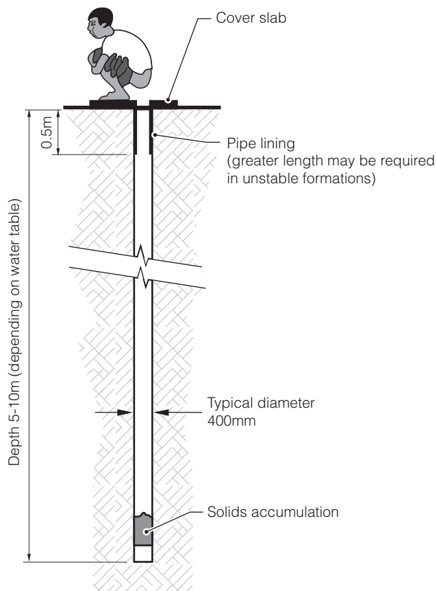
Figure 5.4. Borehole latrine
