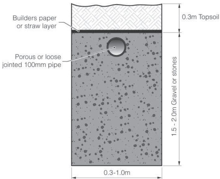
Figure 7.17. Soakfield trench
