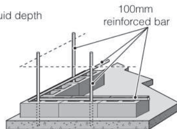
Reinforcement details
