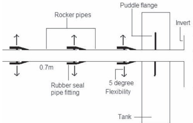
Figure 6.6. Rocker pipes
